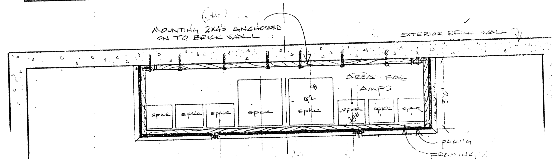
EAST WALL - PLAN & ELEVATION
