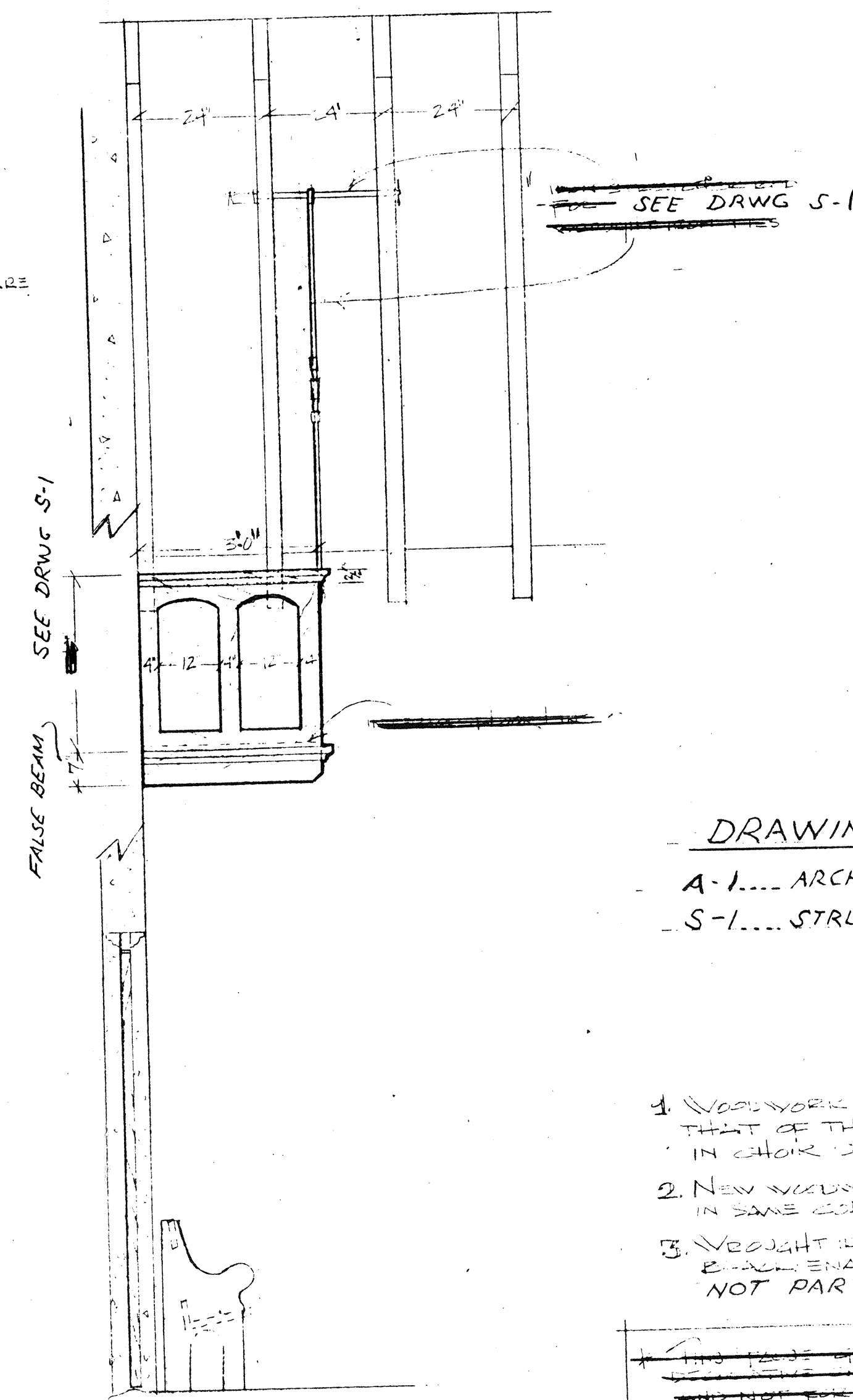
SECTION THRU EAST WALL
